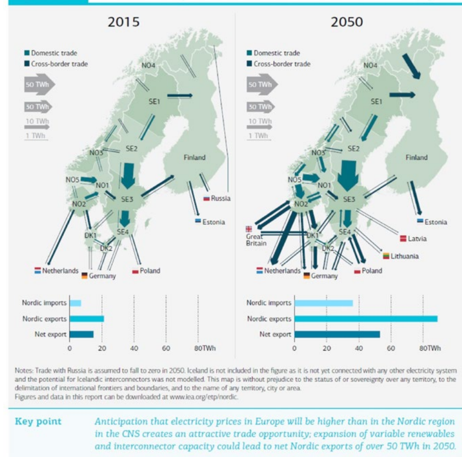
Figure ES.5 Nordic electricity trade in 2015 (left) and 2050 in the CNS (right)
